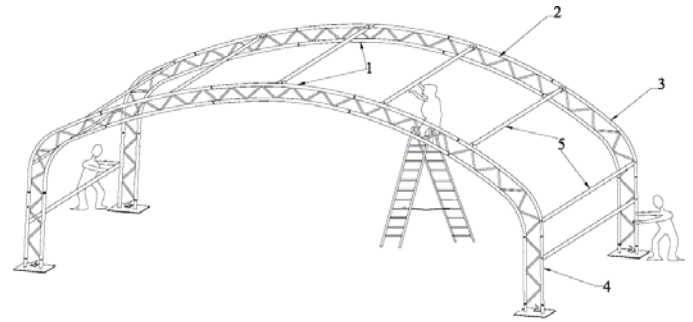
Figure 6 Hint of Installation of arches
