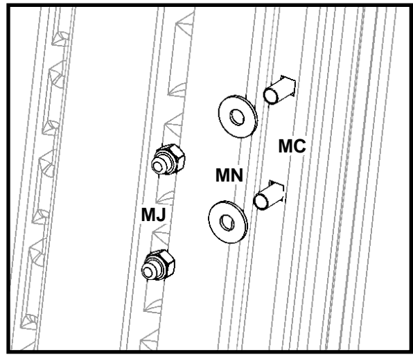
Put Washers (MN) and Cap Nuts (MJ) on Bolts (MC).
